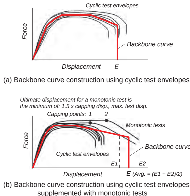
Figure 7-6. Illustration of Backbone Curves Derived from Envelopes of Experimental Test Data
