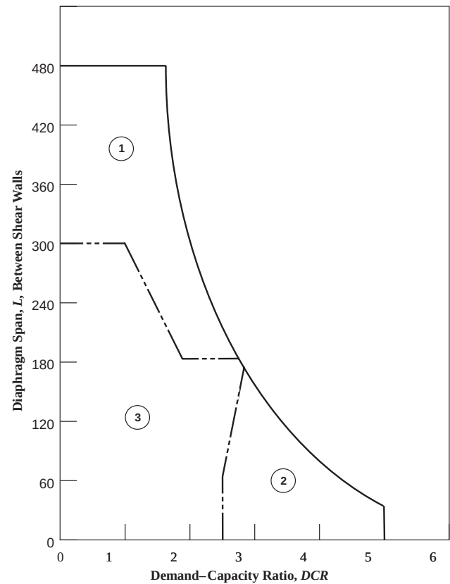
Figure 16-1. Demand–Capacity Ratio for Diaphragms between Shear Walls
