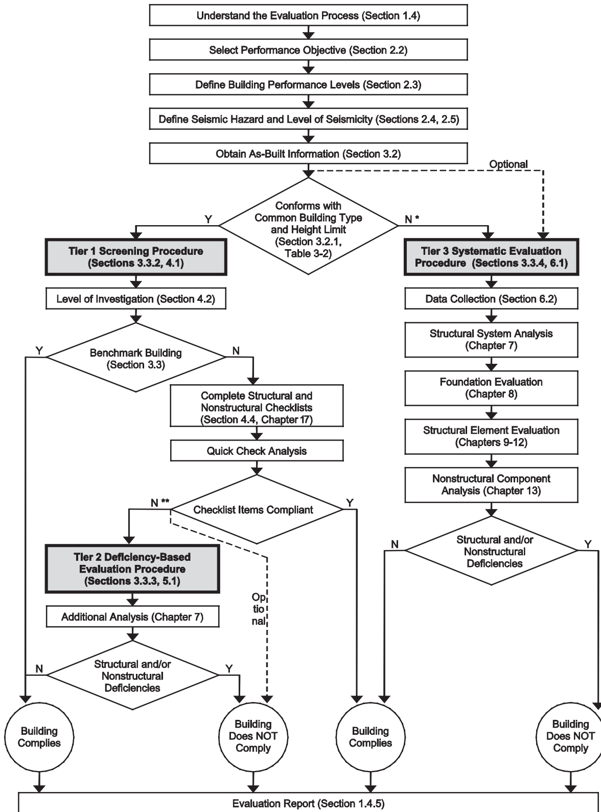
Figure C1-1. Evaluation Process
