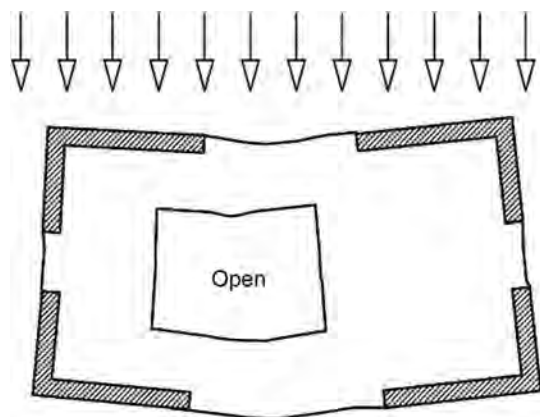
Figure A-35. Diaphragm Opening
