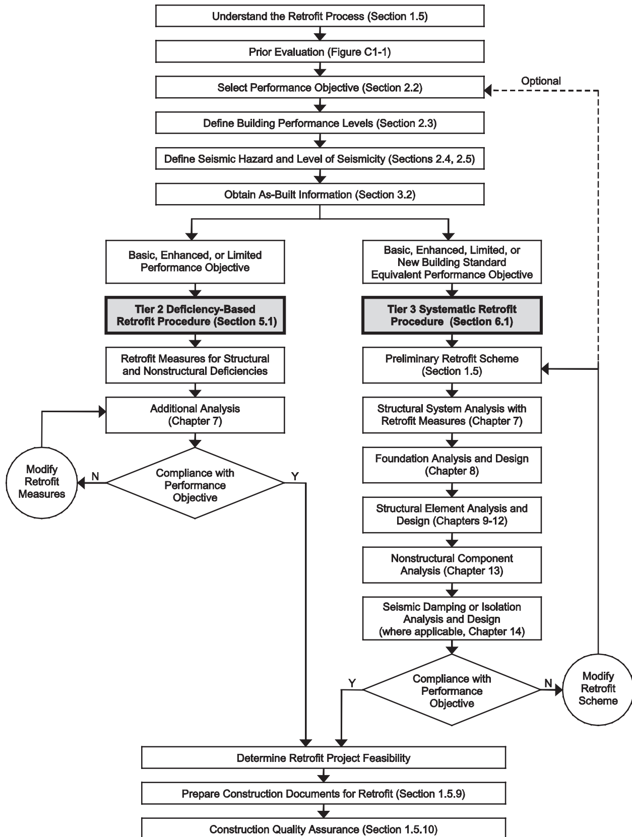
Figure C1-2. Retrofit Process
