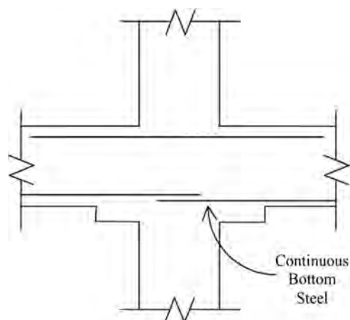
Figure A-16. Continuous Bottom Steel
