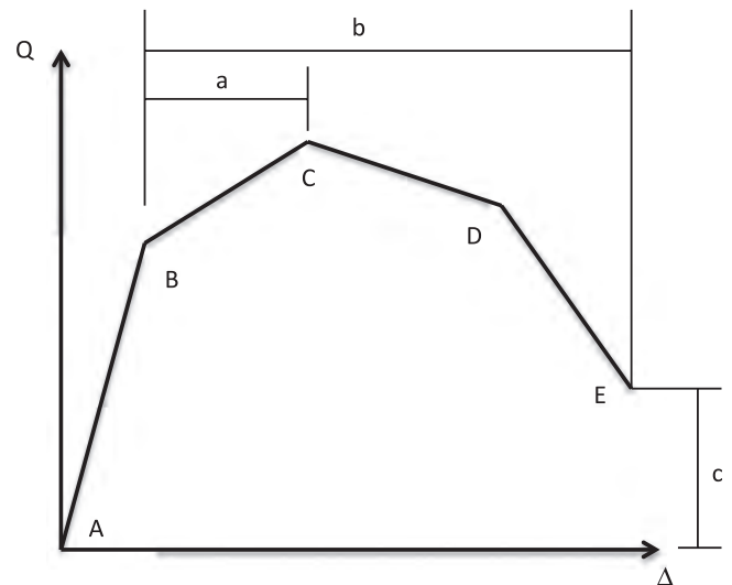
Figure 9-1. Generalized Force-Deformation Relation for Cold-Formed Steel Light-Frame Elements or Components
