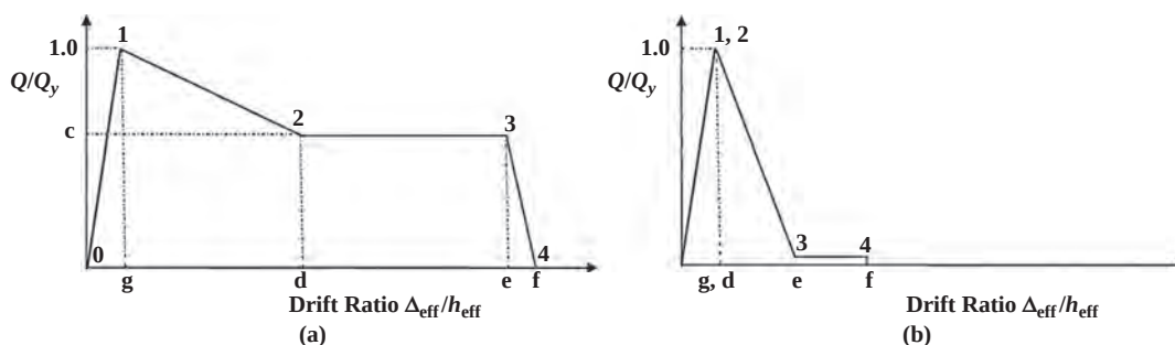
Figure 11-1. Typical Generalized Force. (a) Deformation Relationship for Deformation-Controlled Actions for Reinforced or Unreinforced Masonry; and (b) Deformation Relation for Force-Controlled Actions for Reinforced or Unreinforced Masonry
